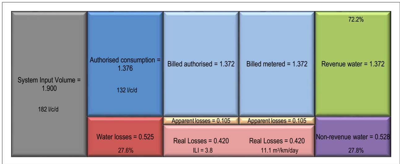
Figure 3: IWA water balance (million m 3 /annum)
