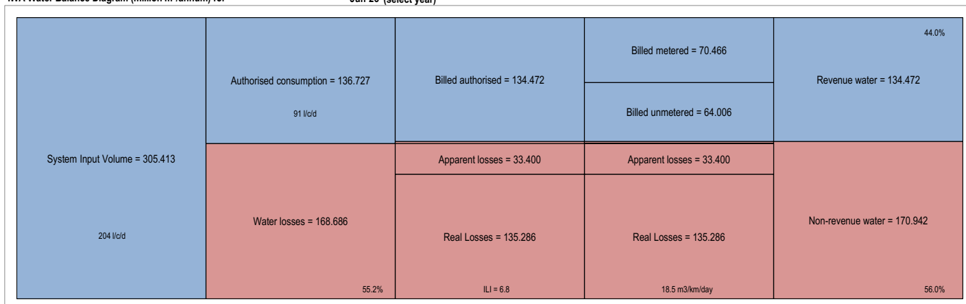
IWA Water Balance Diagram (million m 3 /annum) for Jun-23 (select year)
